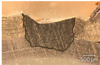
Welding of battery foil stacks consisting of 100 copper foils with TruDisk 2021.
